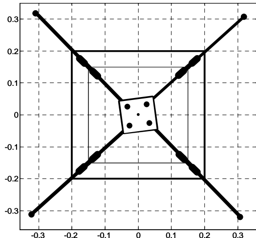
Fig. 6 Scheme: 4RPR parallel robot 'Moving Slide'
