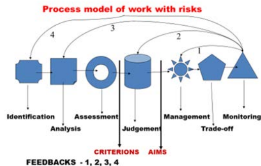
Fig. 3 Process model of work with risks. Criteria = conditions that determined when the risk is acceptable, conditionally acceptable or unacceptable. Aims denote required states. Numbers 1,2,3,4 denote feedbacks that are used if the monitoring shows that followed requirements on safety are not fulfilled [10]
