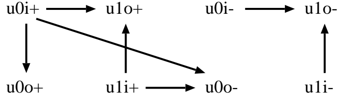
Fig. 9. A reduced signal transition graph for Fig.3 by check-points extraction method
