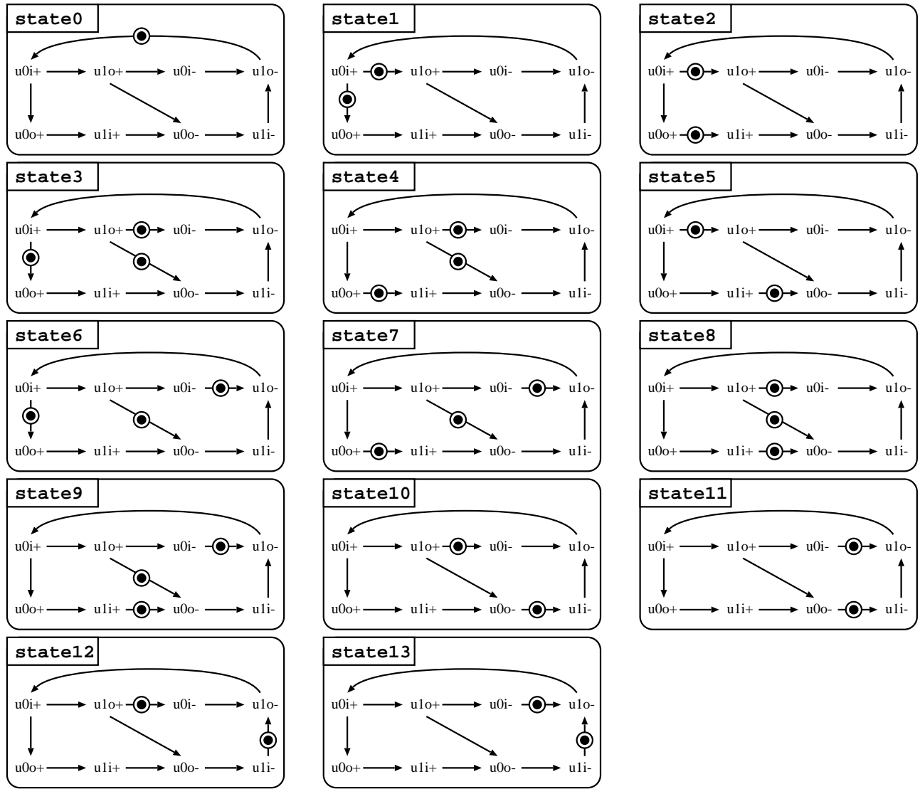
Fig. 5. Firing processes for Fig.3.
