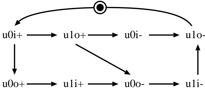
Fig. 3. A signal transition graph for Fig.2
