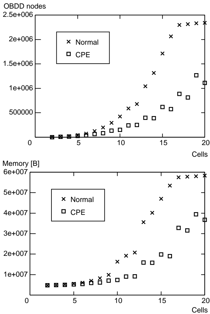
Fig. 12. Verification performance of mutex by NuSMV: OBDD nodes(upper), amount of Memories(lower).
