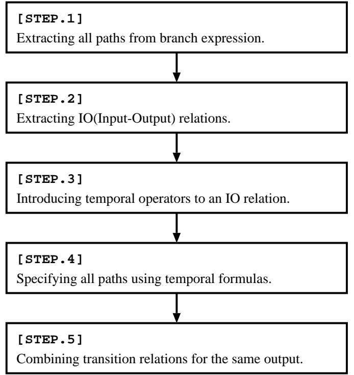
Fig. 8. Procedure of Specification.
