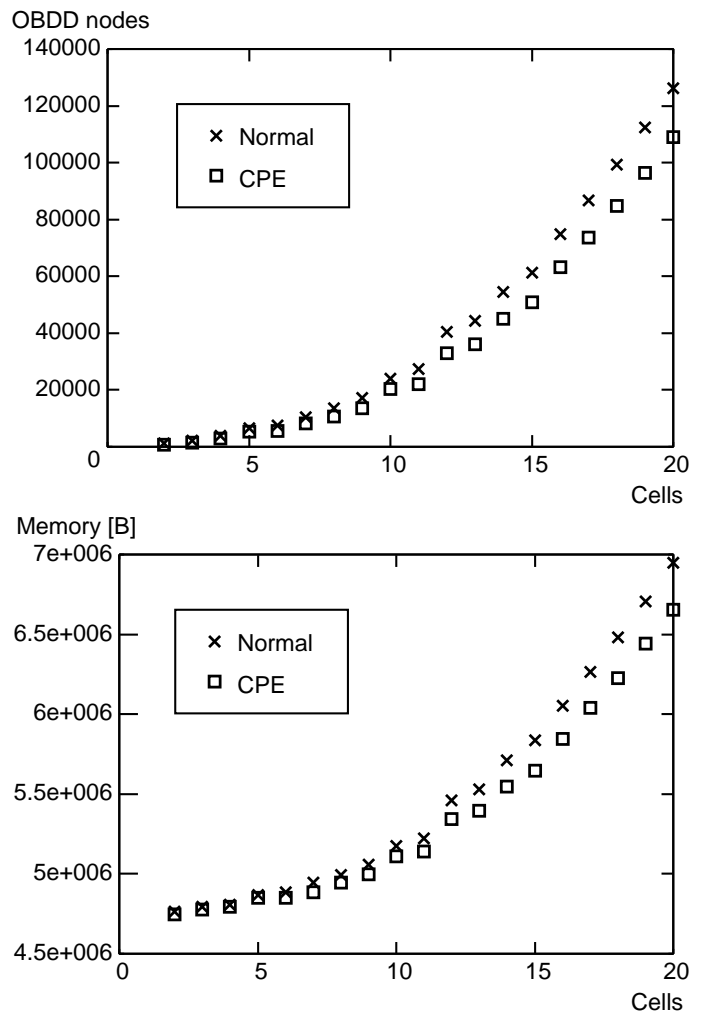
Fig. 11. Verification performance of semaphore by NuSMV: OBDD nodes(upper), amount of Memories(lower).
