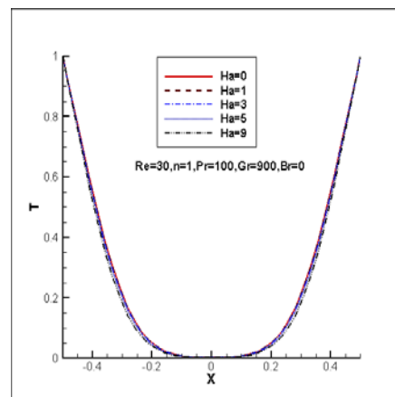
Fig.6. Transient temperature profiles for the different values of Hartman number
