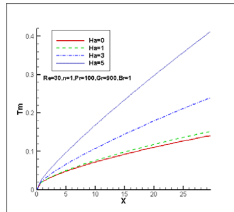
Fig.11. The effect of Hartman number on the mean temperature
