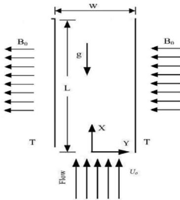
Fig. 1. Geometry and boundary condition
