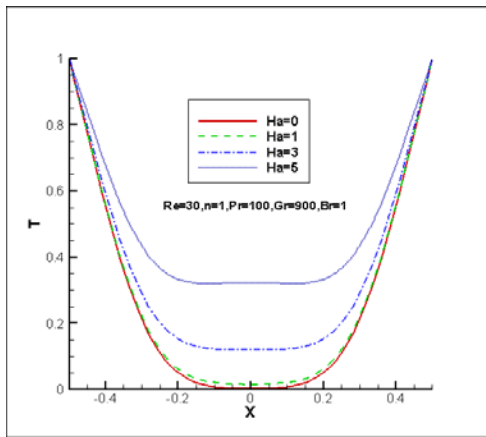
Fig.7. Transient temperature profiles for the different values of Hartman number
