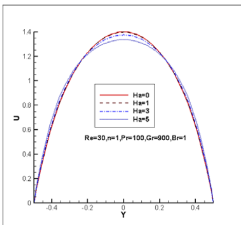
Fig.3. Transient velocity profiles for the different values of Hartman number
