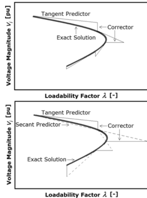
Fig. 1. Predictor/Corrector Mechanism for CLF Analysis [10].
