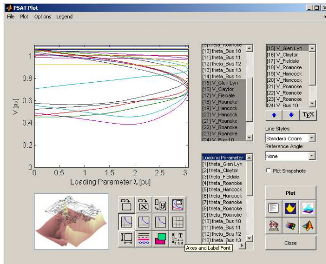
Fig. 9. Nose curves for all network buses of the IEEE 14-bus test system.
