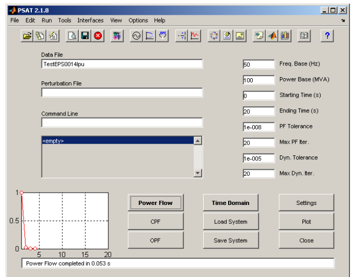
Fig. 5. GUI in PSAT for load flow analysis of IEEE 14-bus system.
