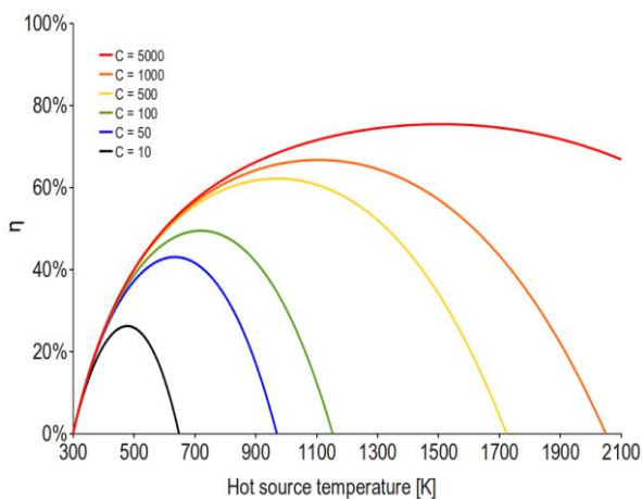
Figure 2: The overall efficiency of the CSP System [9]
