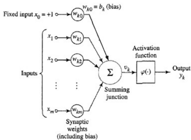
Figure 6. A Sample Neural Network
