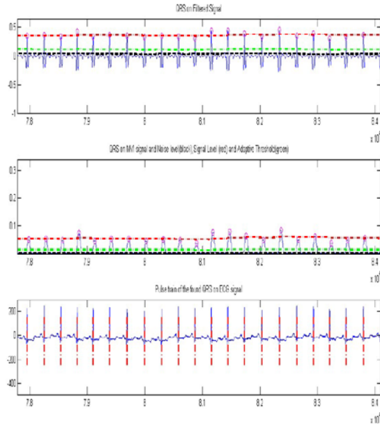
Figure 4. QRS and R-Peaks using Pan Tompkins Algorithm
