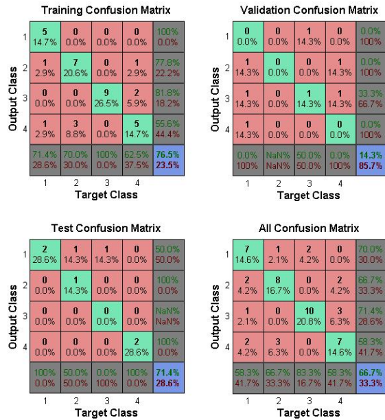
Figure 6. ANN Training for four Classes i.e. Normal, Ventricular Arrhythmia, AV Arrhythmia and Atrial Arrhythmia
