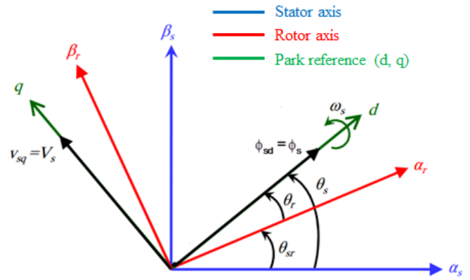
Fig. 6 Orientation of stator flux on the d-axis
