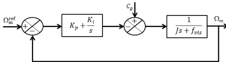
Fig. 5 The speed proportional-integral controller
