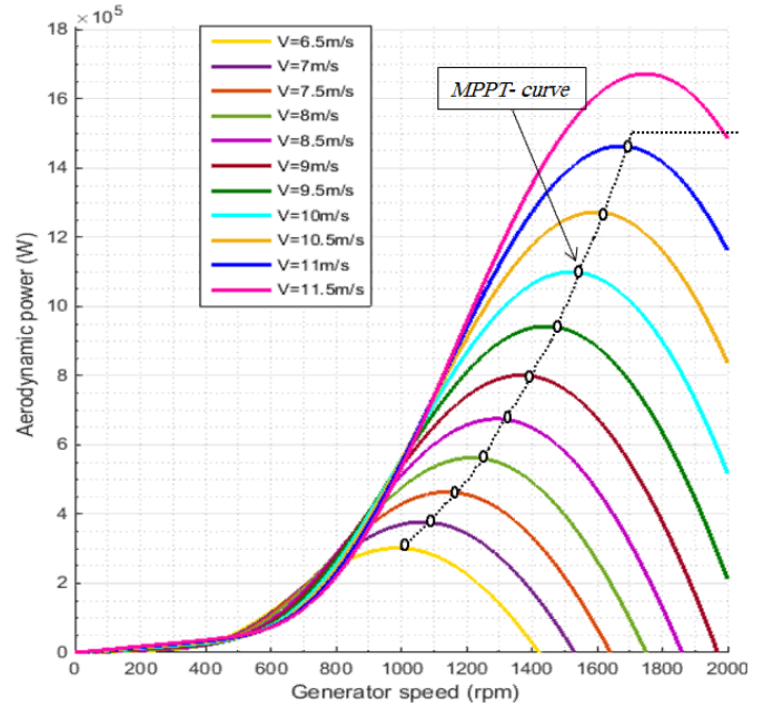
Fig. 3 Optimum operating characteristics of the turbine
