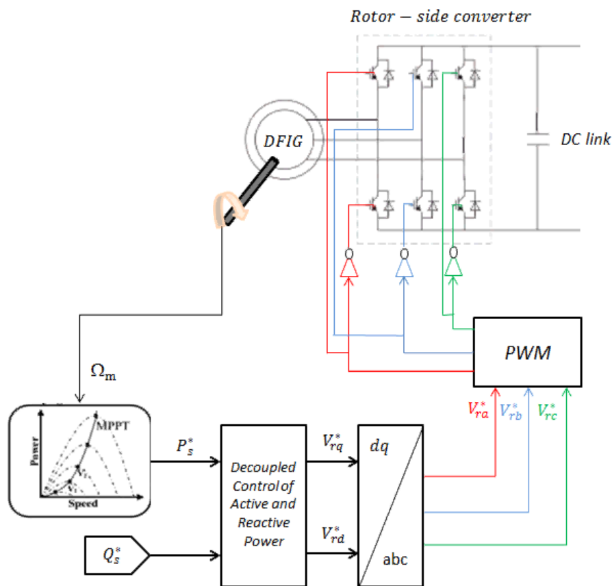
Fig. 8 RSC control diagram
