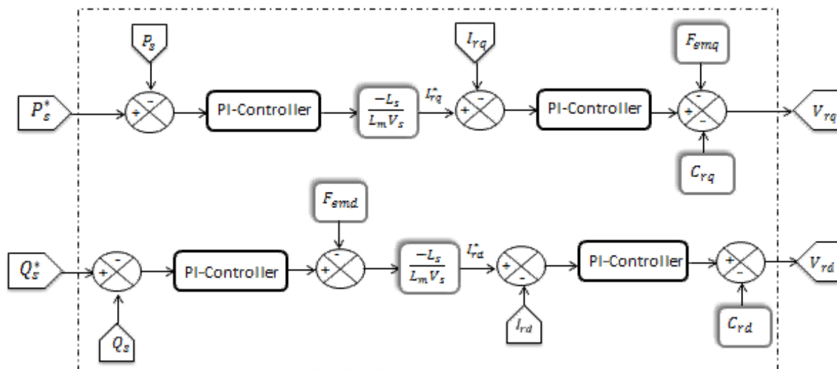
Fig. 10 Direct decoupled control scenario diagram
