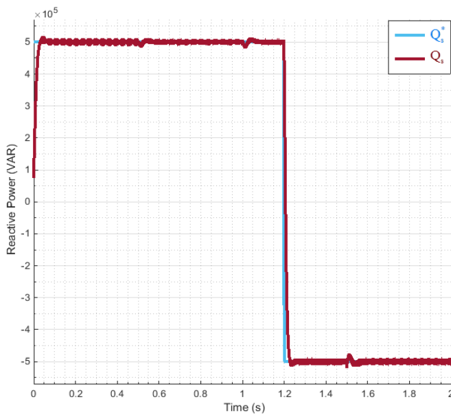
Fig. 12 Stator active and reactive power responses and the rotor currents in the d-q reference
