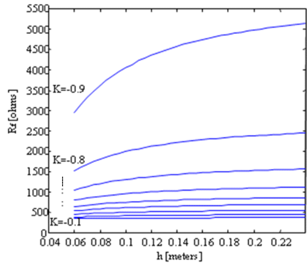
Fig. 6 The map of the relationships of R_f and h , K relation
