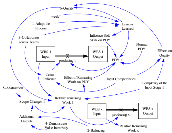
Fig. 7. System Dynamics Model of First (and next “x”) Project Delivery
