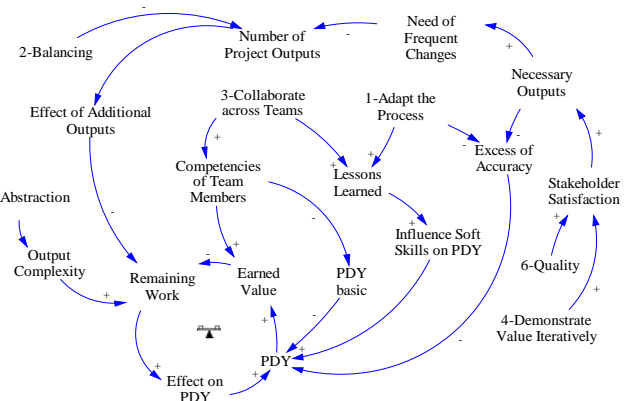
Fig. 4. Causal Loop Diagram of Influence of Iterative Development Key Principles on Cultural Project.
