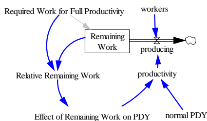
Fig. 5. Level Protected by PDY [14]
