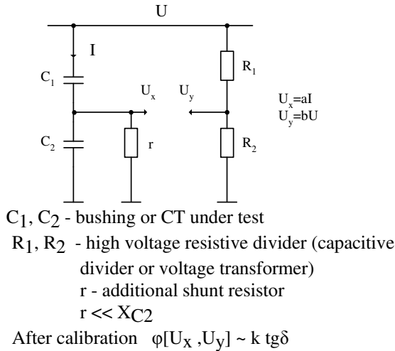
Fig. 4 the measuring diagram
