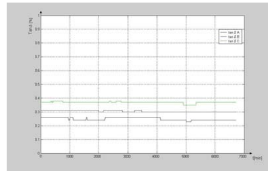
Figure 8 the time variation of \tan \delta at the bushings on the outputs of 400 kV
