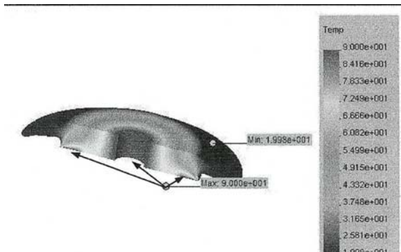
Figure 14 temperature distribution on a radial section
