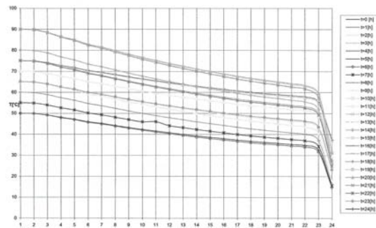
Figure 13 temperature variation on the elements of the 123 kV, 1600 A bushing, for a given operation time
