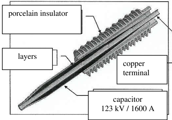
Figure 10 the 123 kV, 1600 A isolated outdoor bushing
