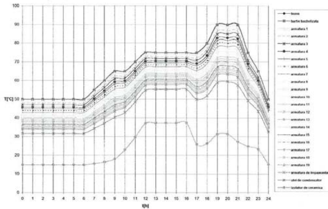
Figure 15 temperature variation on the elements of the 123 kV, 1600 A bushing
