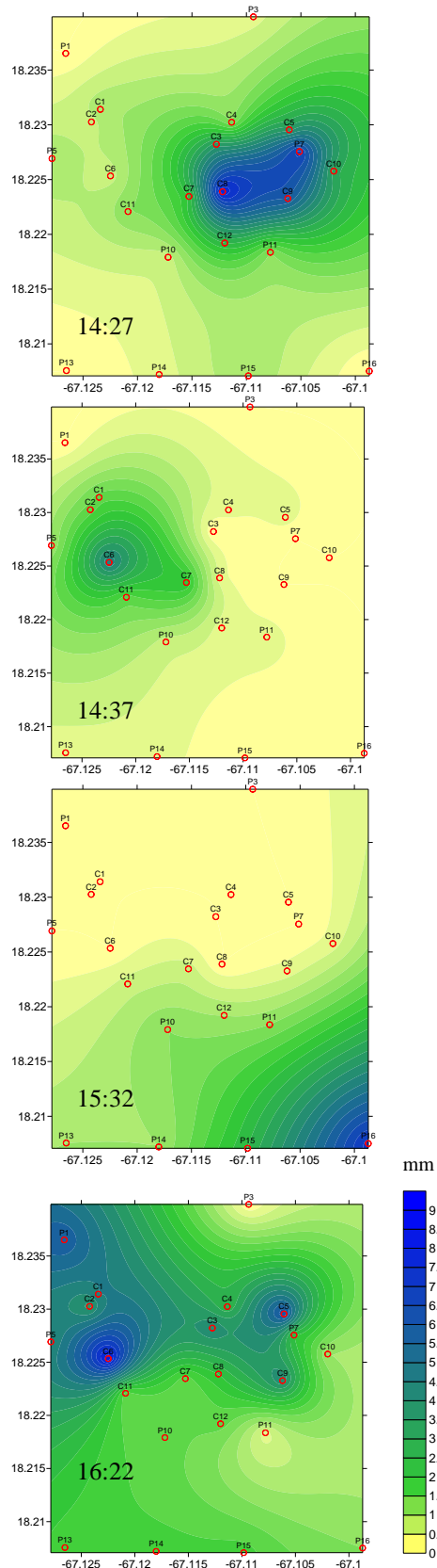
Figure 5. Spatial distribution of 5-minute rainfall values (mm) at 14:27, 14:37, 15:32 and 16:22 hours, for a storm occurring on 27 June, 2007.
