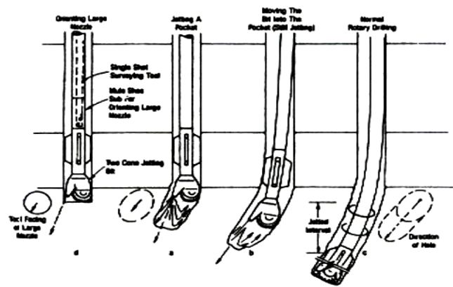
Fig. 1. Jetting bit technique
