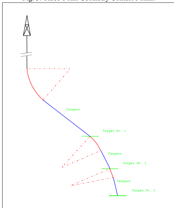
Fig. 6. Single Circular Arc Trajectories.
