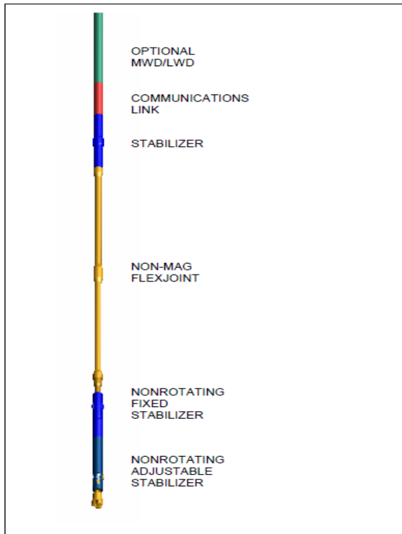
Fig. 4. NAS Bottom Hole Assembly.
