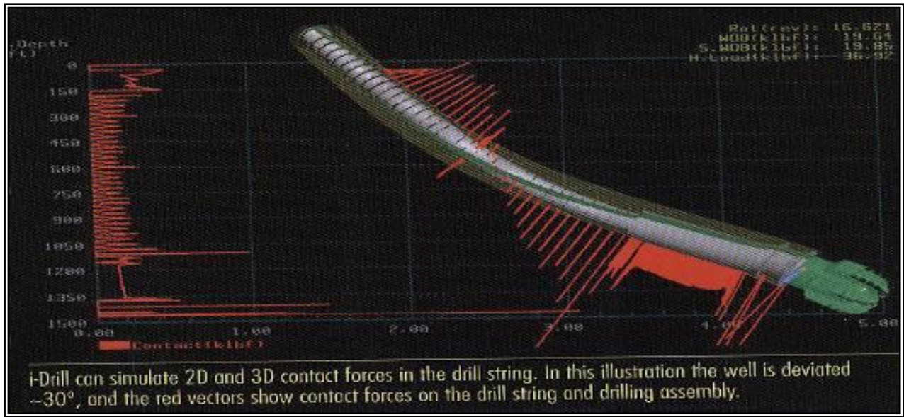
Fig. 9. Contact forces on the drill string and drilling assembly
