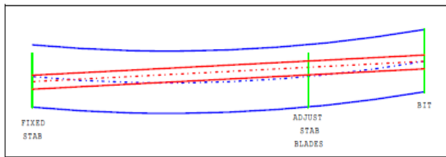
Fig. 5. Three-Point Geometry Contact Points.
