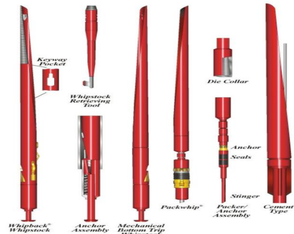
Fig. 2. Whip Stocks & Whip Stock Mills
