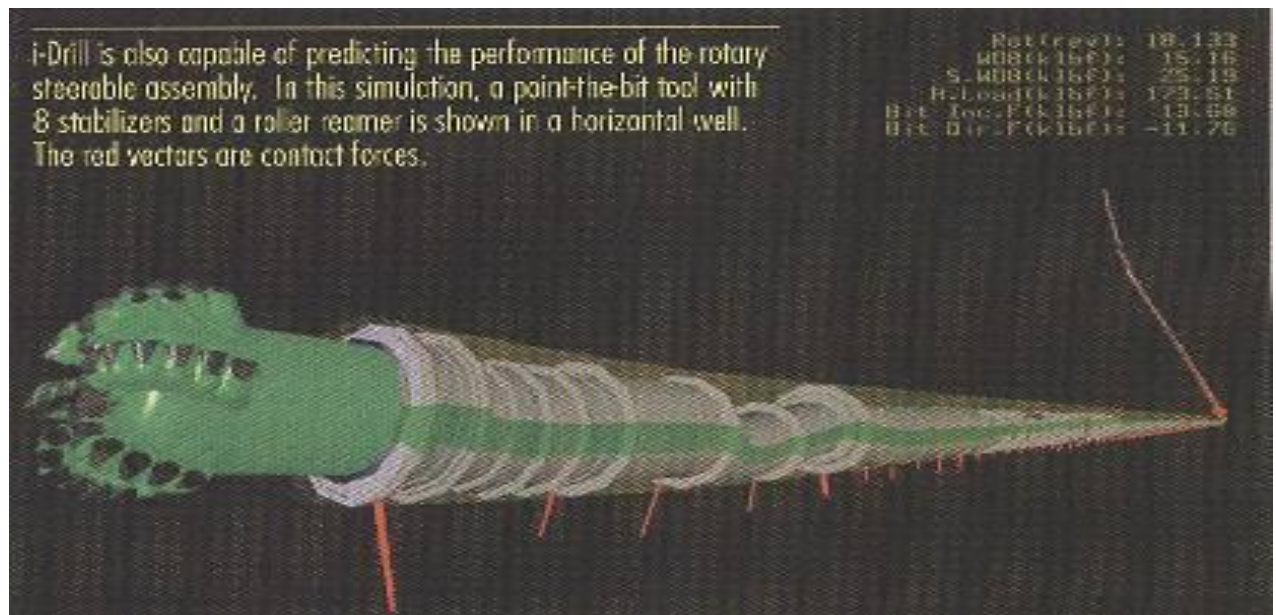
Fig. 10. predicting the performance of the rotary steerable assembly
