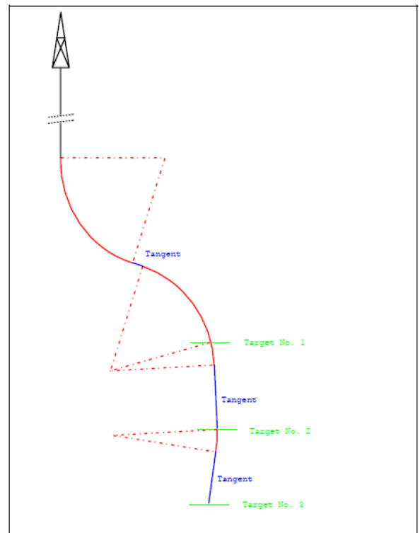
Fig. 7. Two Circular Arc Trajectory.
