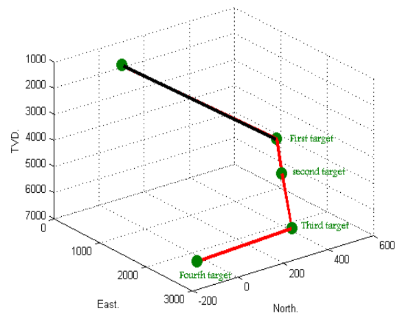
Fig. 9. Simulate Four Target Directional at First Target.
