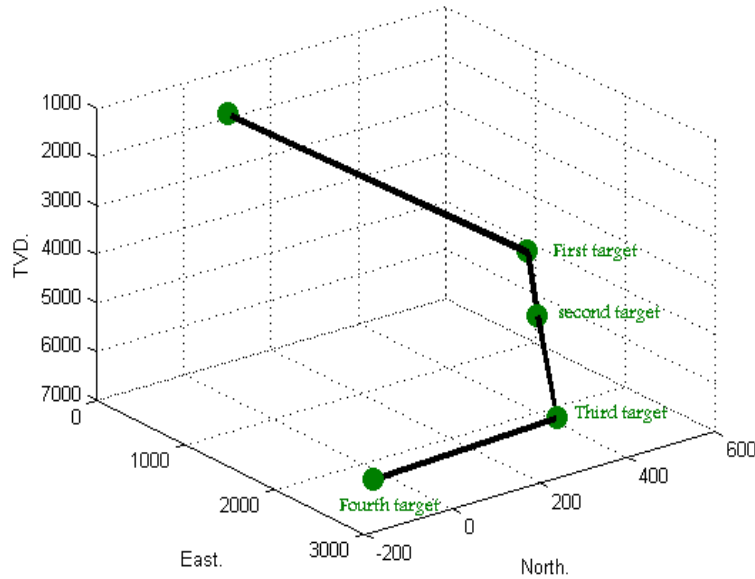
Fig. 10. Simulate Four Target Directional at Total Depth.
