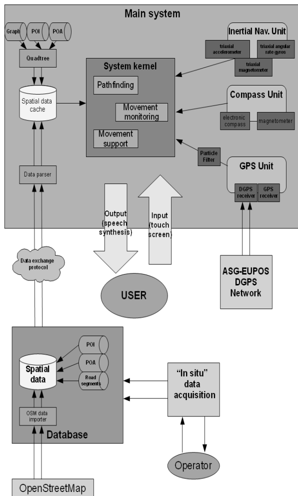
Fig. 4. Architecture of the system
