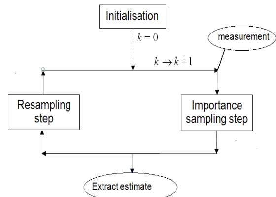
Fig. 11. Particle Filter Diagram
