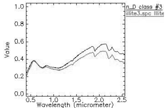
Fig. 9 identification of illite
