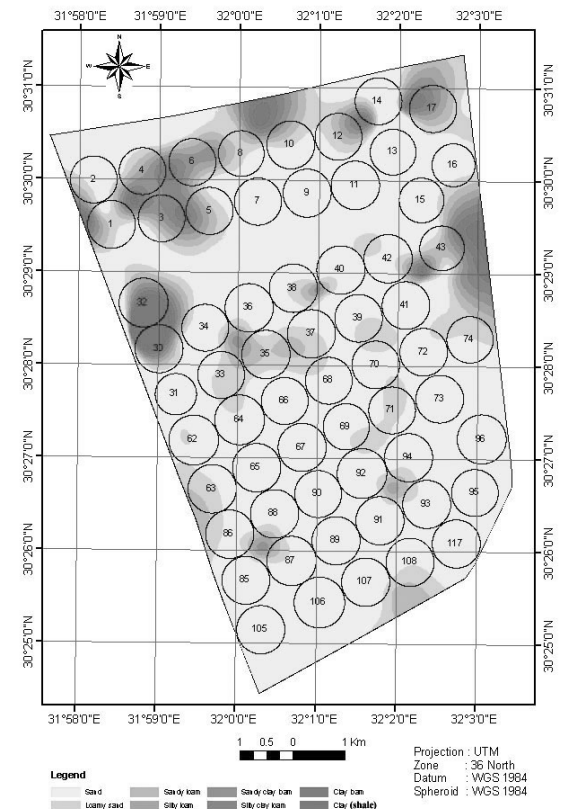
Fig.5 Spatial variability of shale distribution
