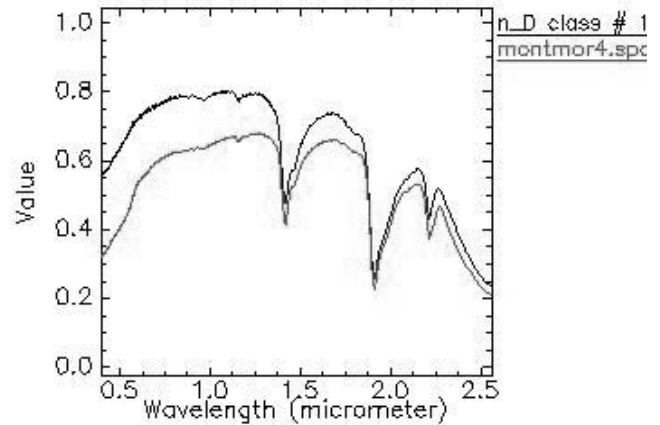
Fig. 7 identification of montmorillonite
