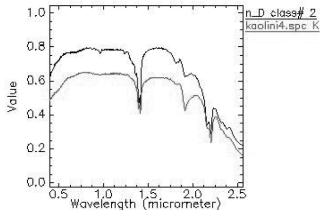
Fig. 8 identification of kaolinite
