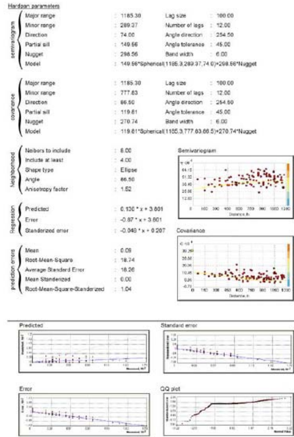
Fig. 4 shows spatial variability parameters
