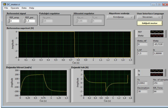
Fig. 4 Control desk
