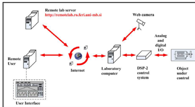
Fig. 3 Architecture of the Remote Laboratory
