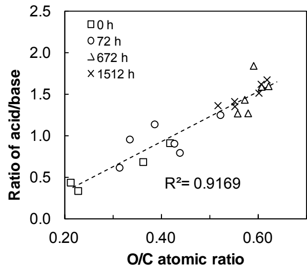
Figure 11 Correlation of the acidity to basicity ratio (A/B) with the oxygen to carbon atomic ratio (O/C) for heat-treated jack pine wood during weathering
