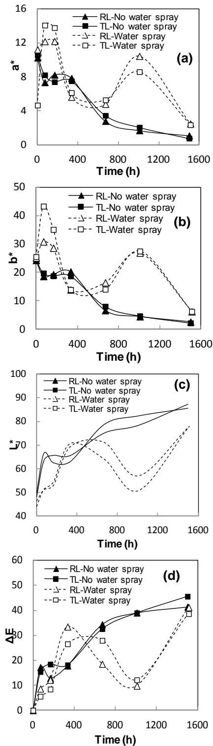
Figure 3 Color changes of heat-treated jack pine during different weathering conditions, reported using CIE-L*a*b* system: (a) red/green coordinate ( a^* ), (b) yellow/blue coordinate ( b^* ), (c) lightness coordinate ( L^* ), (d) total color difference ( \Delta E )
